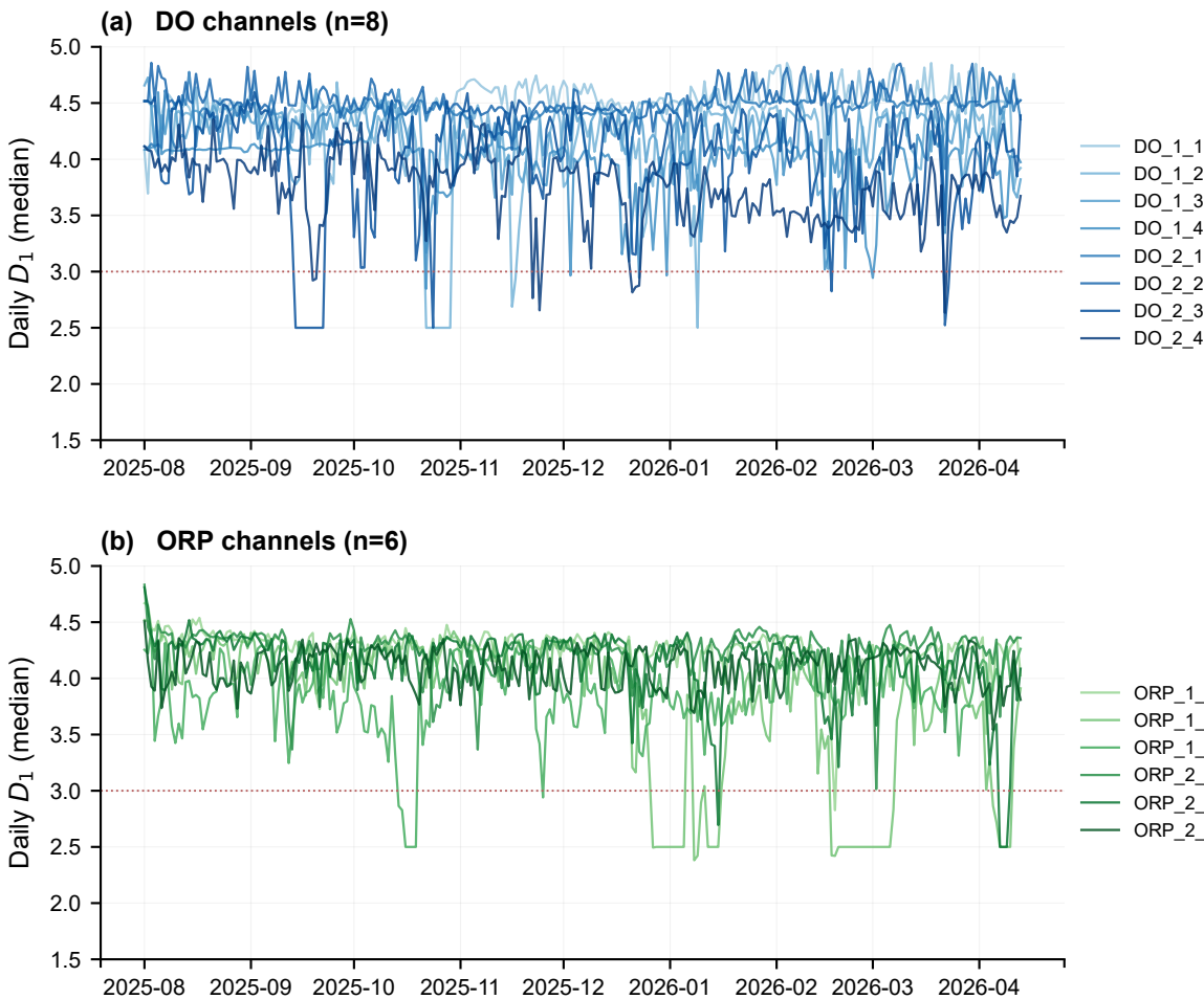
Figure 7. Daily D_1 trajectories by sensor group (final, DO/ORP only)
